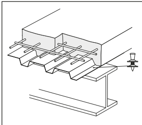
Floor decking
