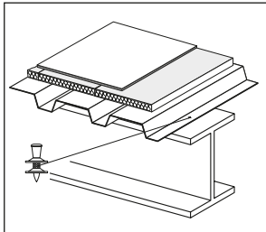
Roof decking
