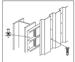
Wall liners
